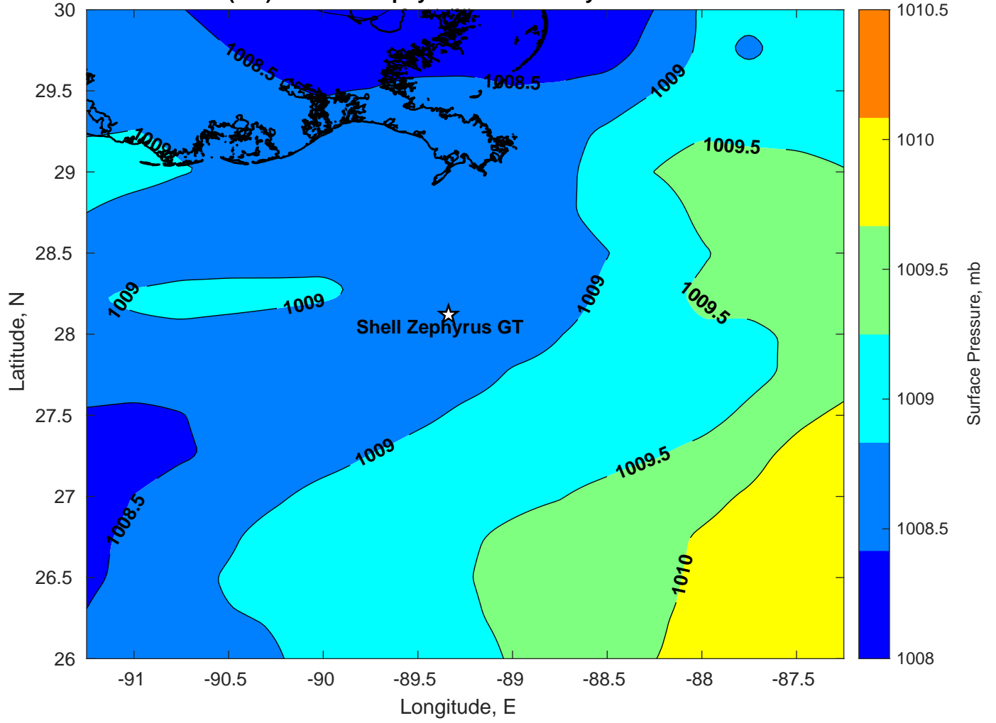
Surface Pressure (mb) for Shell Zephyrus GT at 10-May-2024 06:00:00
